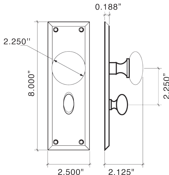
8801-250 Large Oval Knob, Small Rose
