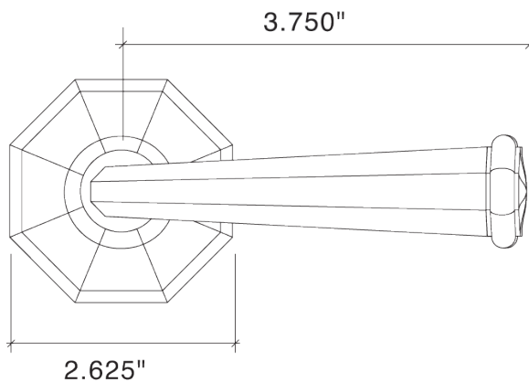
Small Moorestown Lever 8834 Large Moorestown Rose 8858-262
