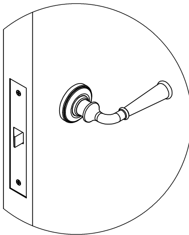
9101 Interior Mortise Lock Shown with Non-Suited Section Trim & 8821 Lever (Lever High Configuration)
